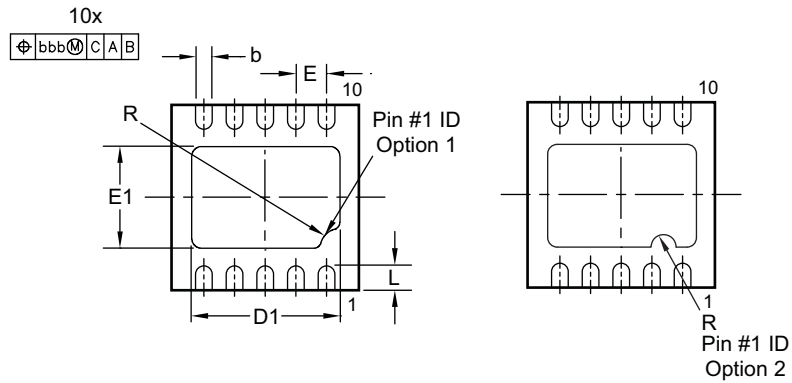
BOTTOM VIEW
