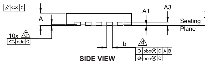
SIDE VIEW
