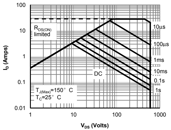
Figure 12: Maximum Forward Biased Safe Operating Area for AOTF7T60L (Note F)
