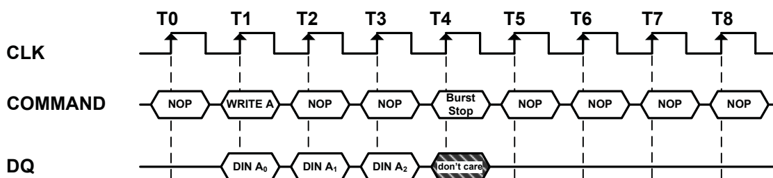
Figure 17. Termination of a Burst Write Operation (Burst Length = X)
