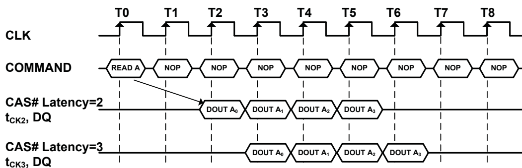
Figure 4. Burst Read Operation (Burst Length = 4, CAS# Latency = 2, 3)
