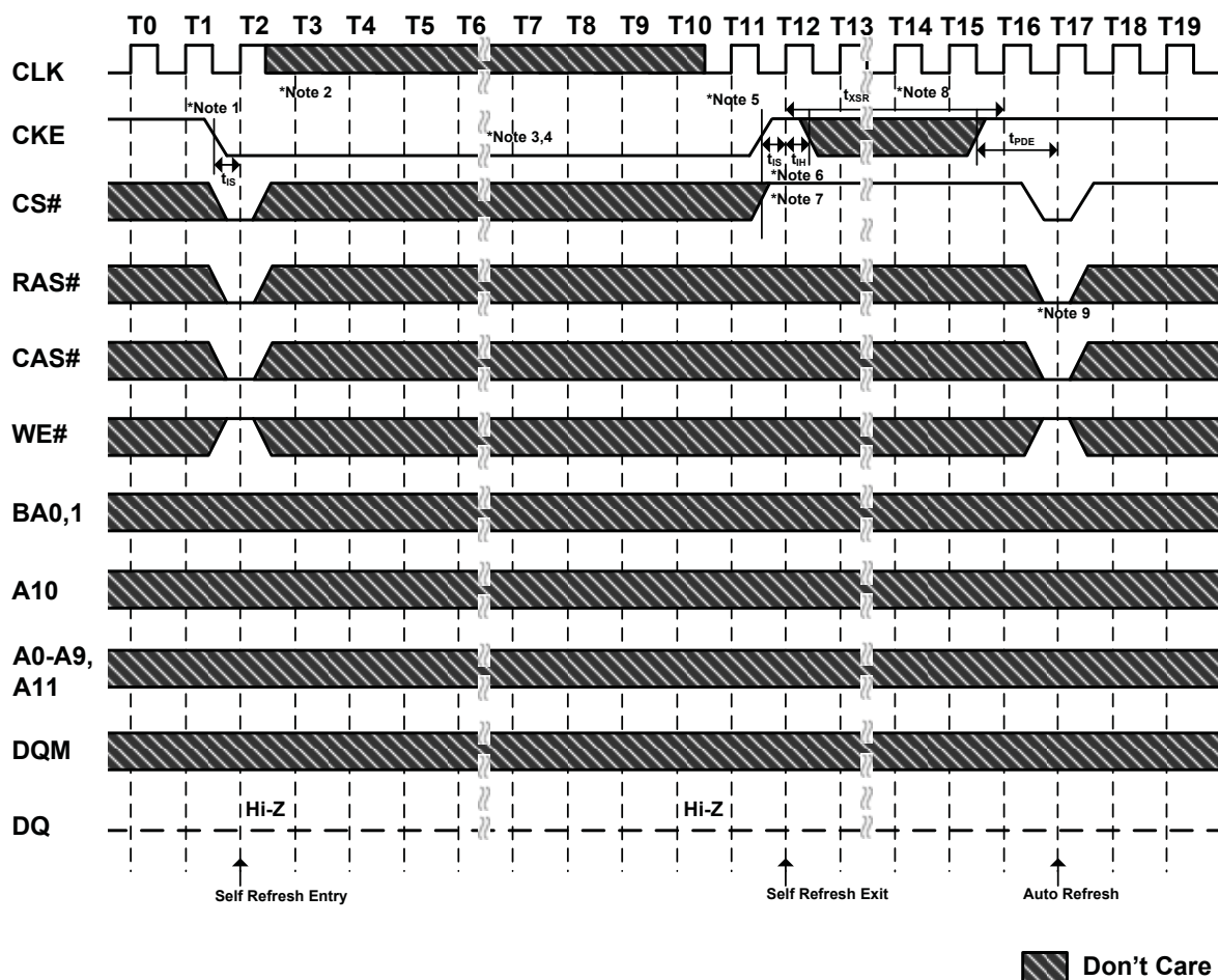
Figure 23. Self Refresh Entry & Exit Cycle
