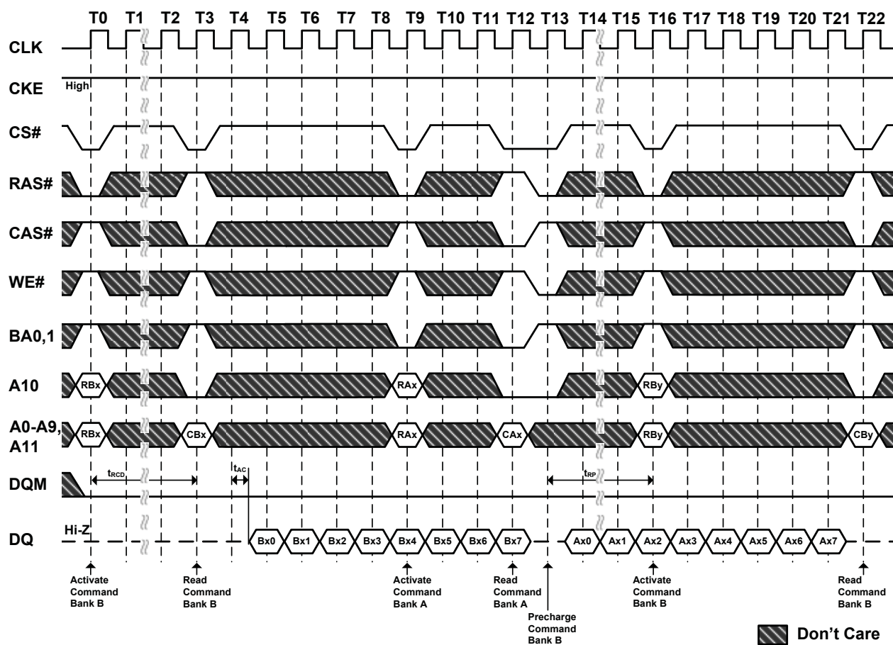
Figure 29.1. Random Row Read (Interleaving Banks) (Burst Length=8, CAS# Latency=2)
