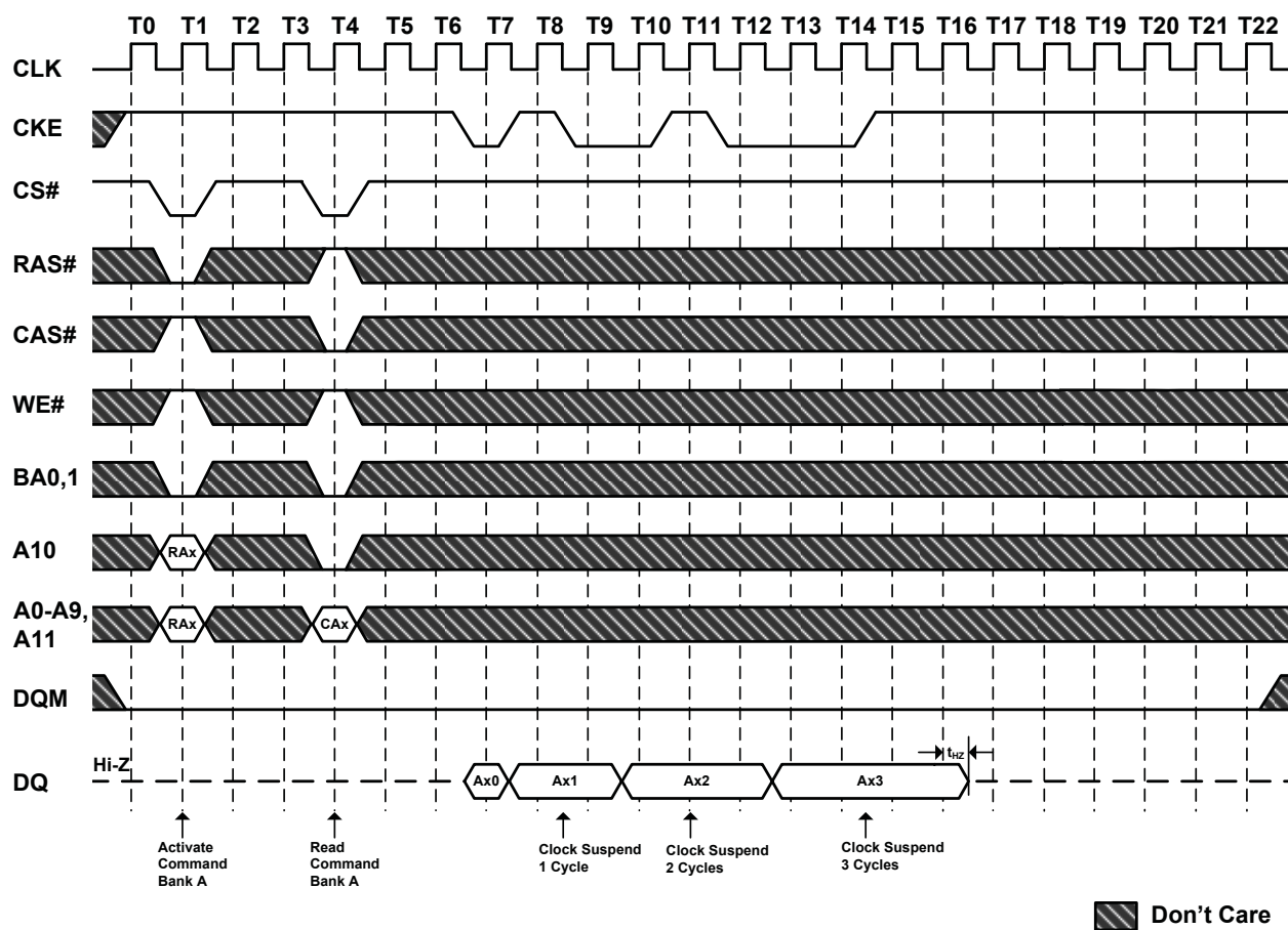
Figure 24.2. Clock Suspension During Burst Read (Using CKE) (Burst Length=4, CAS# Latency=3)
