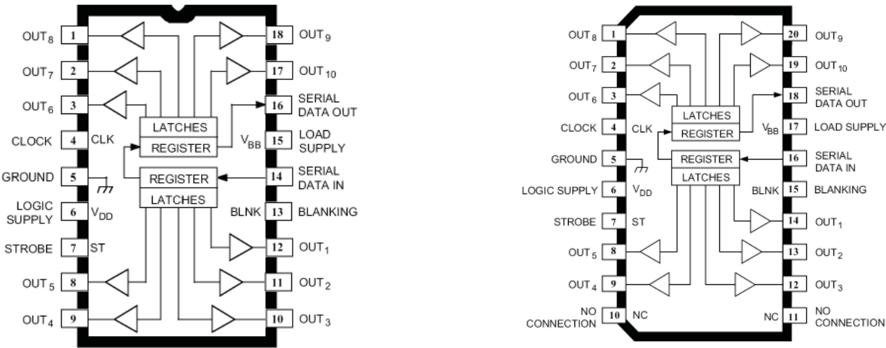
Pin-out Diagrams
