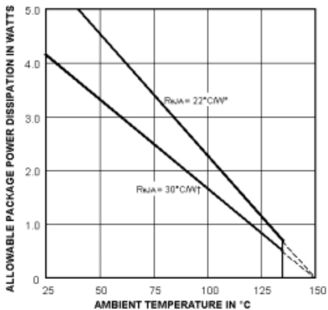
A3935KED (PLCC)
