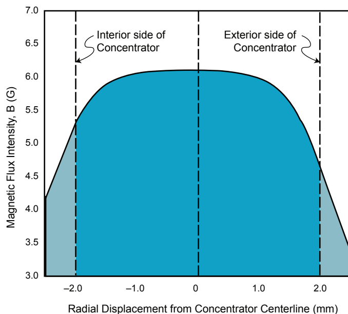
Figure 9. Side view of example current-conducting wire and split ring concentrator (left), and magnetic profile (right) through the midplane of the gap in the split ring concentrator. The flux density through the center of the gap varies between the inside and the outside of the gap.
