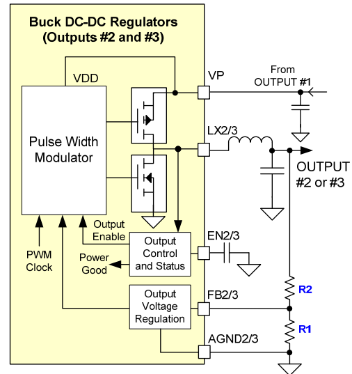
Figure 10 - Power Outputs #2, #3 Block Diagram
