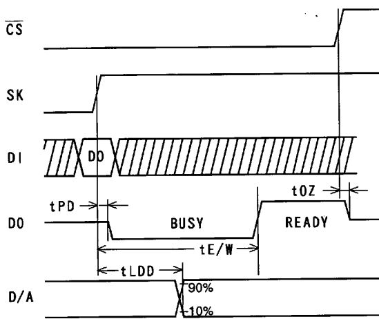
READY/ \overline{\text{BUSY}} signal output timing
