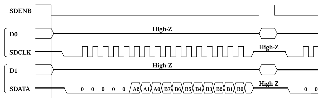
Fig. 22 Register Write Operation
