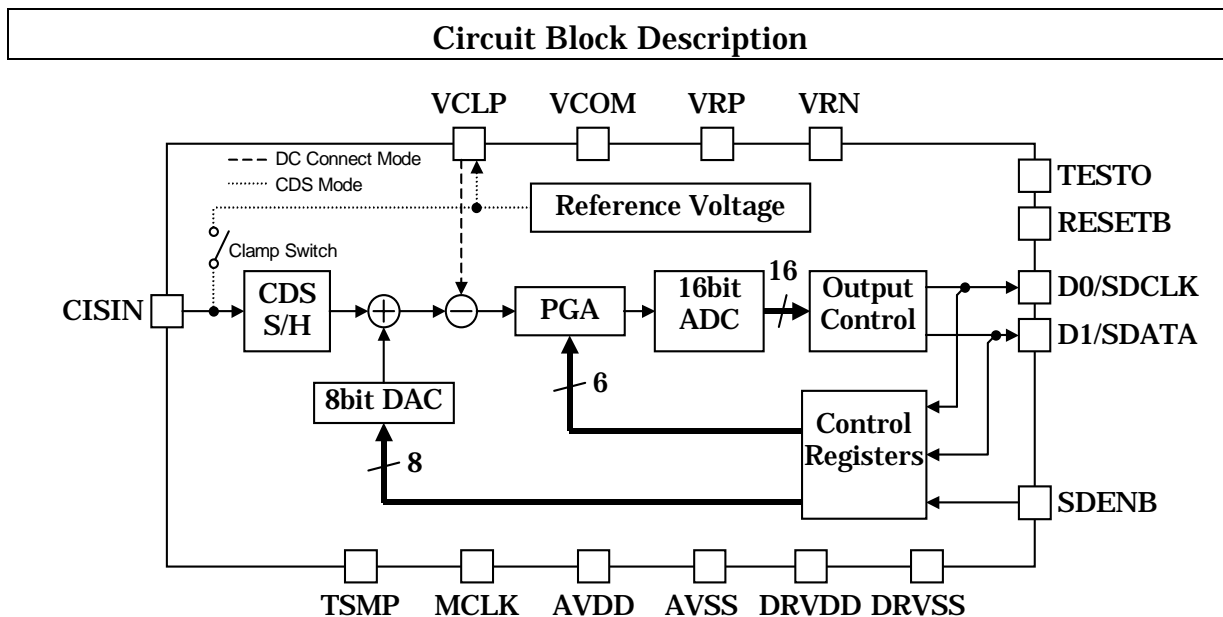
Fig. 1 Block Diagram
