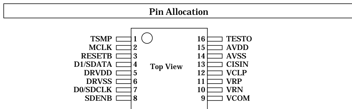
Fig. 2 Pin Allocation
