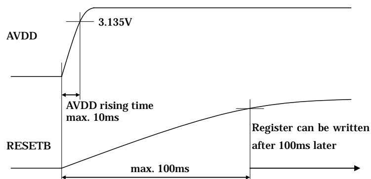
Fig. 9 Power-On-Reset
