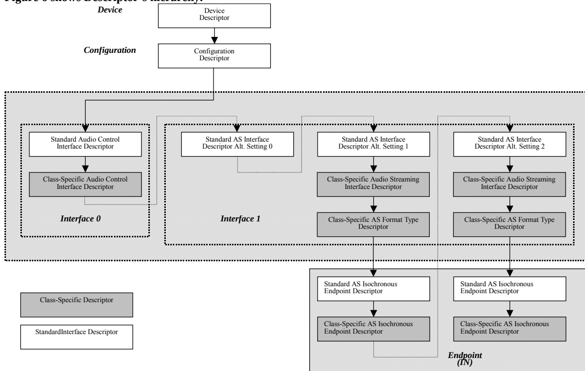
Figure 6. Descriptor Hierarchy
