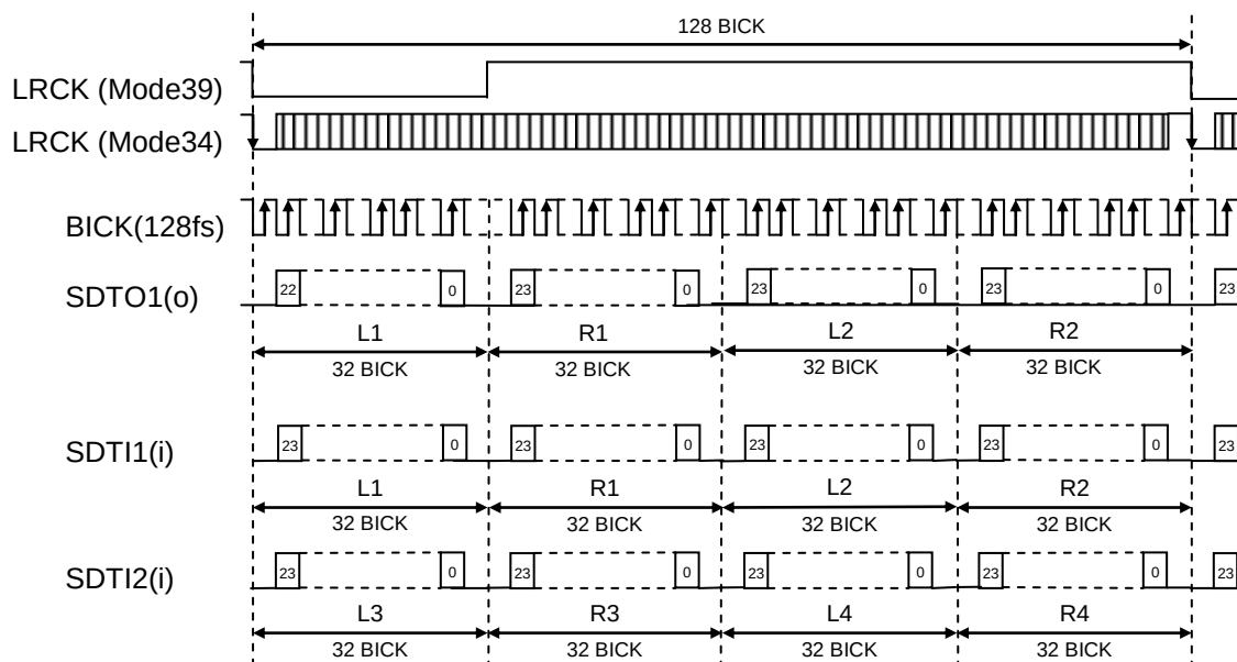
Figure 42. Mode 34/39 Timing (TDM128 Mode)
