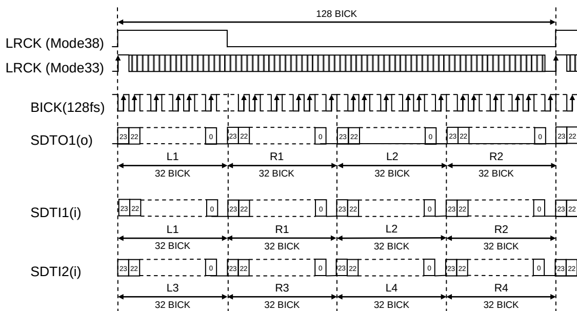
Figure 41. Mode 33/38 Timing (TDM128 Mode)
