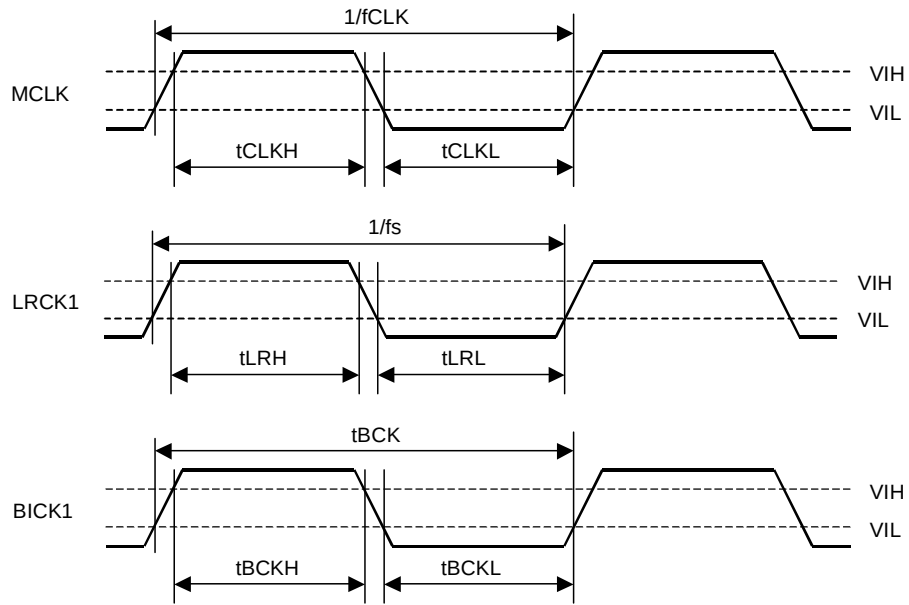
Clock Timing (TDM 256 mode, TDM 128 mode)
