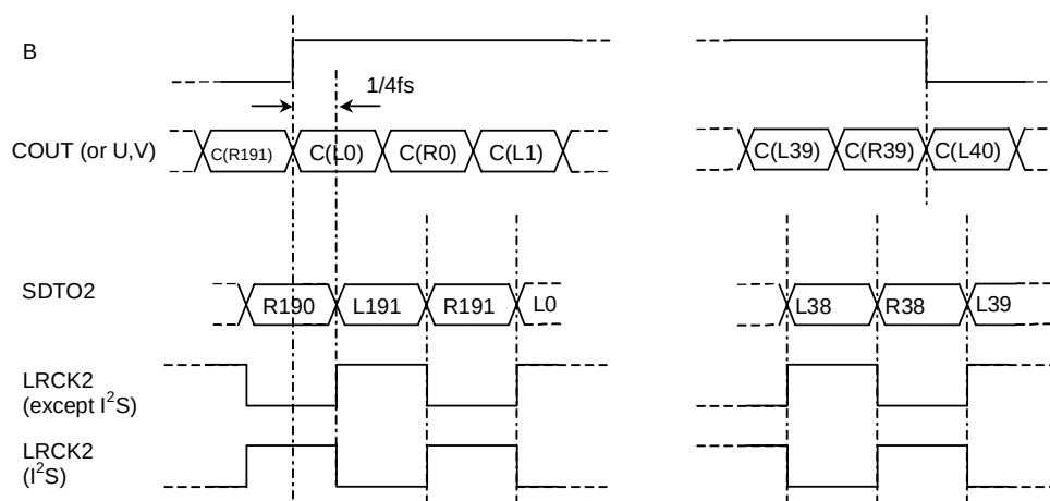
Figure 21. B, C, U, V output/input timings
