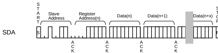
Figure 47. WRITE Operation
