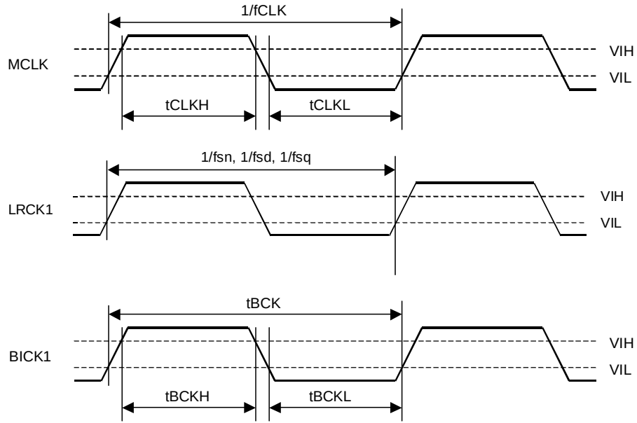
Clock Timing (Normal mode)
