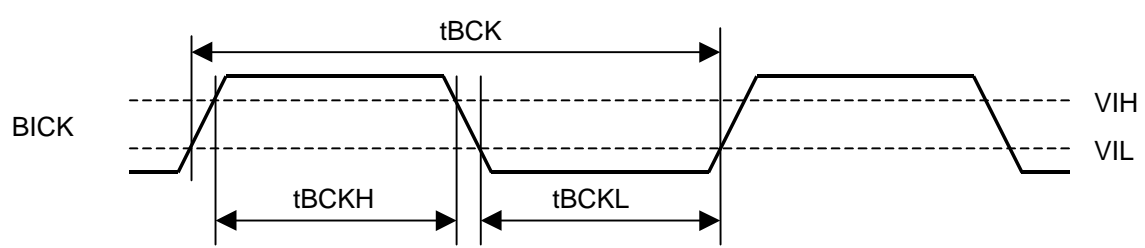
Clock Timing
