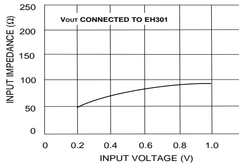
INPUT IMPEDANCE AS A FUNCTION OF INPUT VOLTAGE
