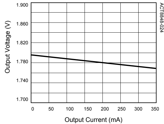
REG12 Output Voltage vs. Output Current
