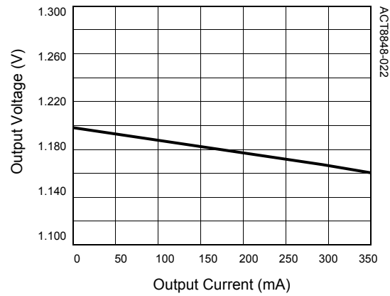
REG10 Output Voltage vs. Output Current
