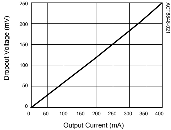
REG10/11/12 Dropout Voltage vs. Output Current
