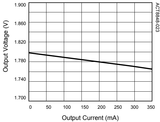
REG11 Output Voltage vs. Output Current
