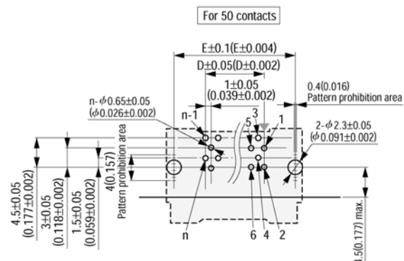
Printed Circuit Board Layout (Component Side View)
