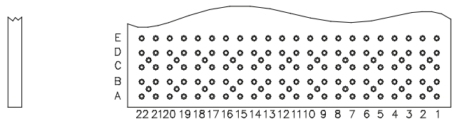
Recommended PCB hole mounting pattern for row differential applications. (Same geometry as above without the ground vias.)
