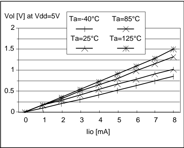
Figure 87. Typical V_{OL} at V_{DD}=5V ( \overline{RESET} )
