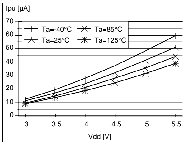
Figure 78. Typical I_{PU} vs. V_{DD} with V_{IN} = V_{SS}
