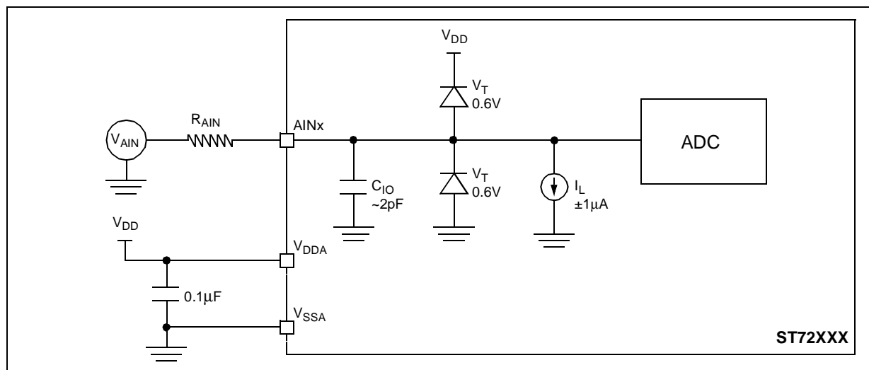
Figure 94. Typical Application with ADC
