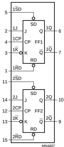
Fig.4 Functional diagram.
