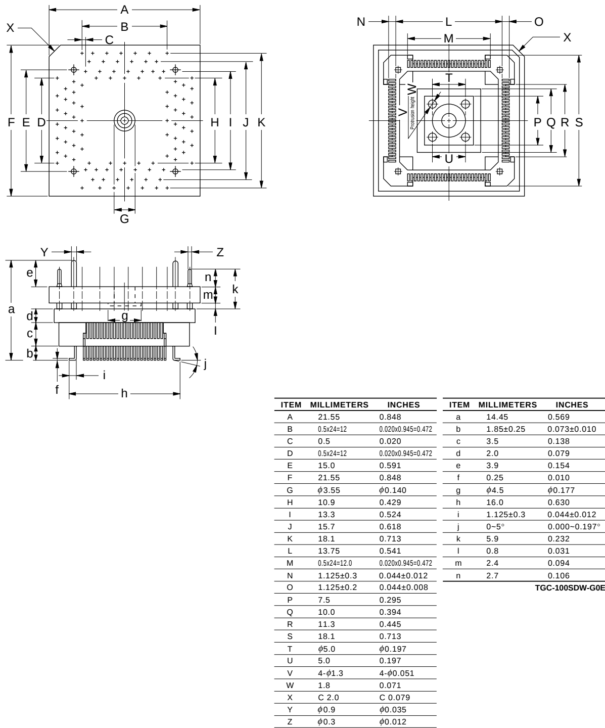
Figure A-3. Drawings of TGC-100SDW (for reference only) (Unit: mm)
