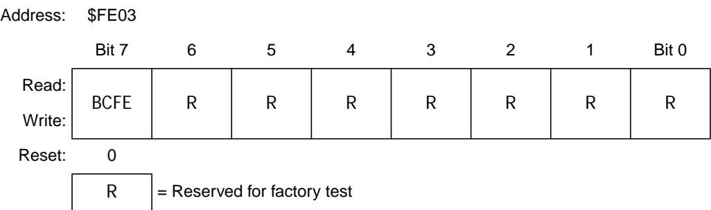
Figure 7-17. SIM Break Flag Control Register (SBFCR)
