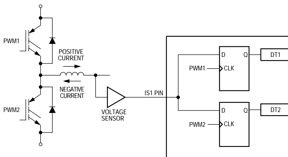
Figure 9-22. DTx bits
