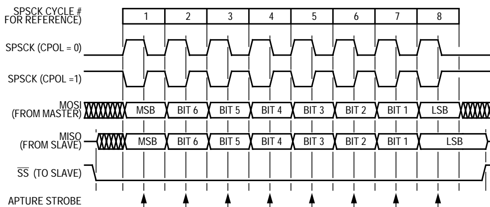
Figure 13-6. Transmission Format (CPHA = 1)
