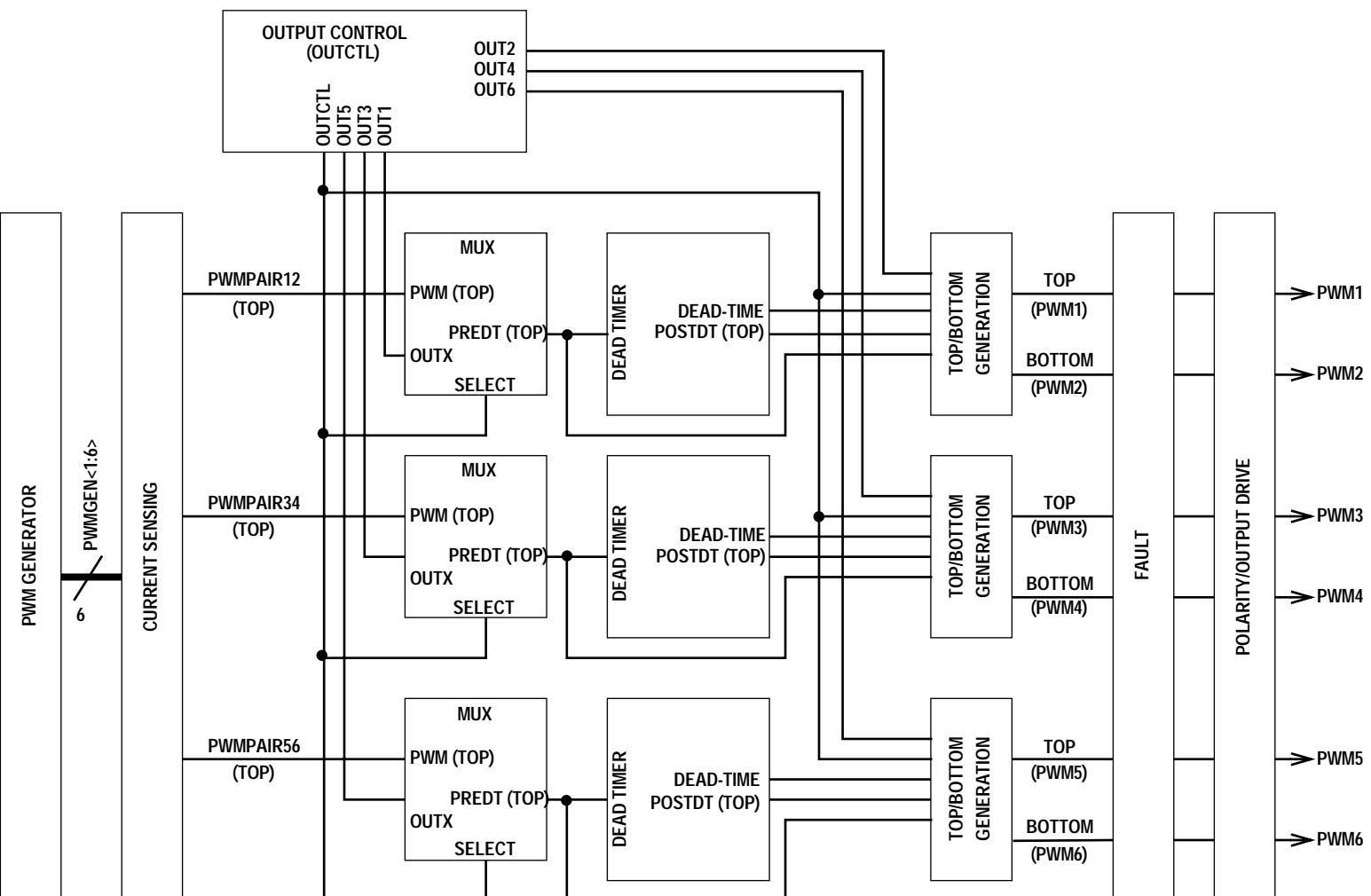
Figure 9-13. Dead-Time Generators
