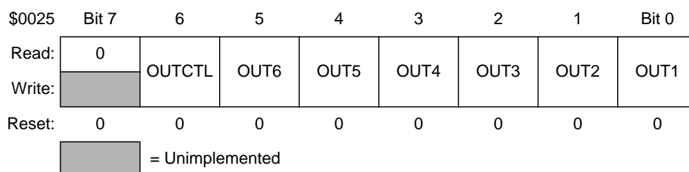
Figure 9-28. PWM Output Control Register (PWMOUT)
