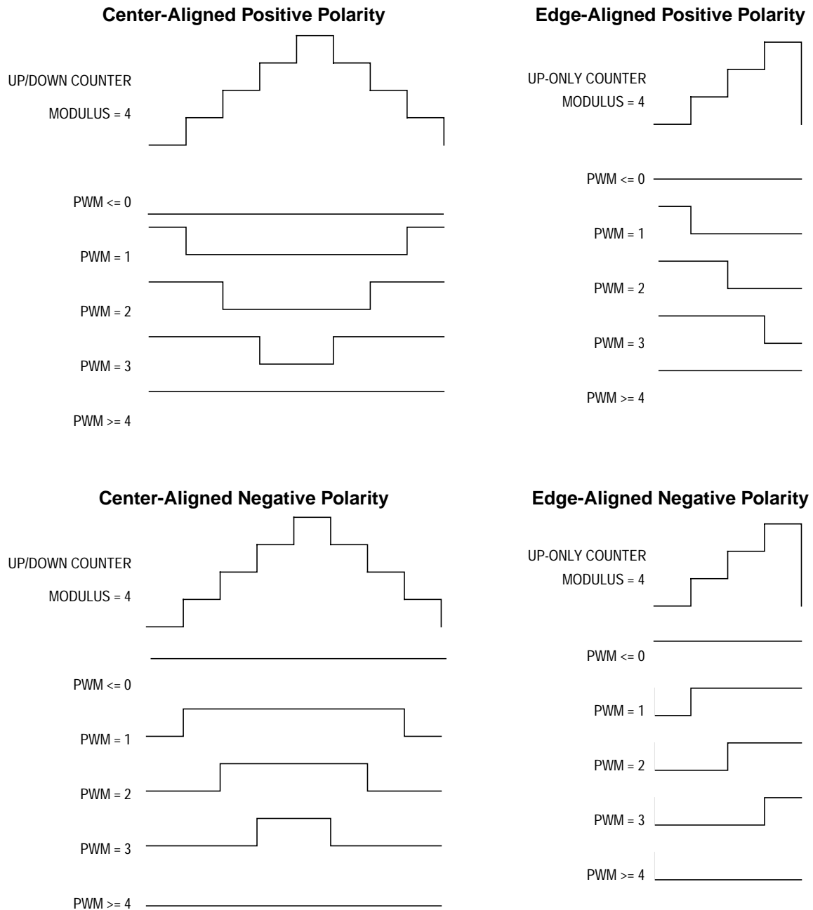
Figure 9-27. PWM Polarity
