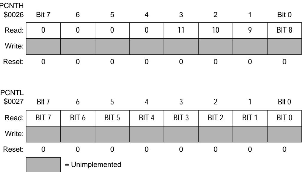
Figure 9-40. PWM Counter Registers (PCNTH:PCNTL)
