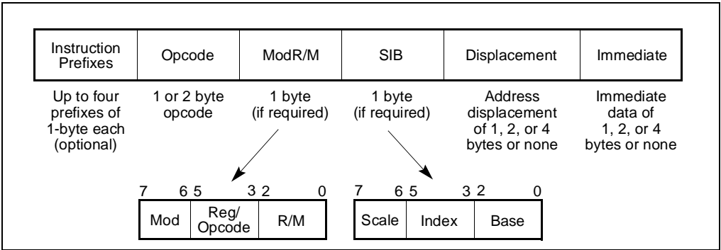
Figure 11-1. Instruction Format
