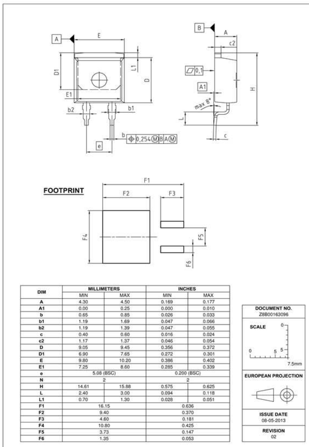
Figure 1 Outlines TO-263-2, dimensions in mm/inch
