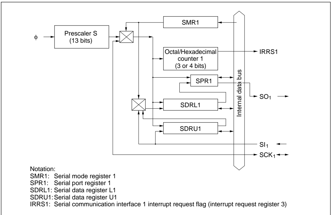
Figure 10-1 Block Diagram of SCII1
