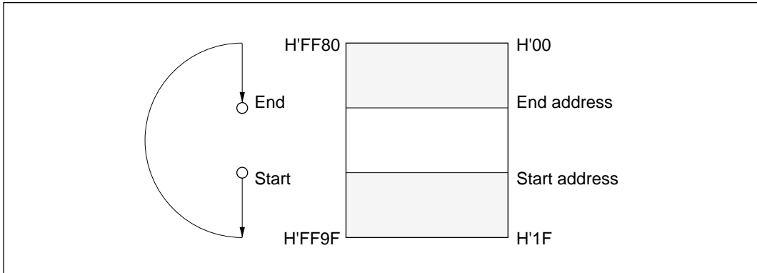
Figure 11-2 Operation When Start Address Exceeds End Address
