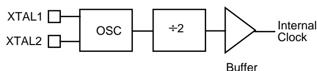
Figure 3-1. Z8 Clock Circuit
