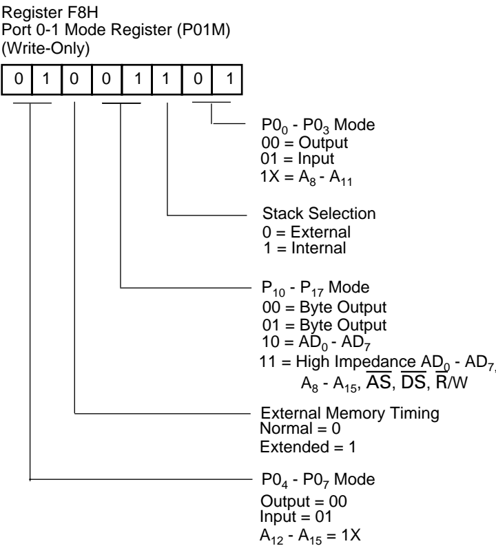
Figure 5-27. Port 0/1 Reset
