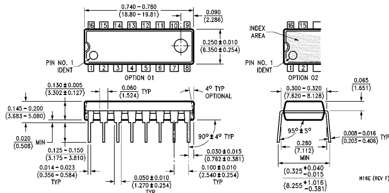
Molded Dual-In-Line Package (N) Order Number CD4518BMN, CD4518BCN, CD4520BMN or CD4520BCN NS Package Number N16E
