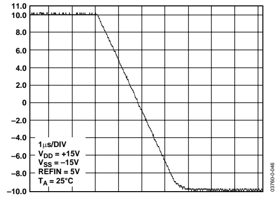
Figure 27. Settling Time
