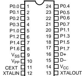
24-pin SOIC/QSOP
