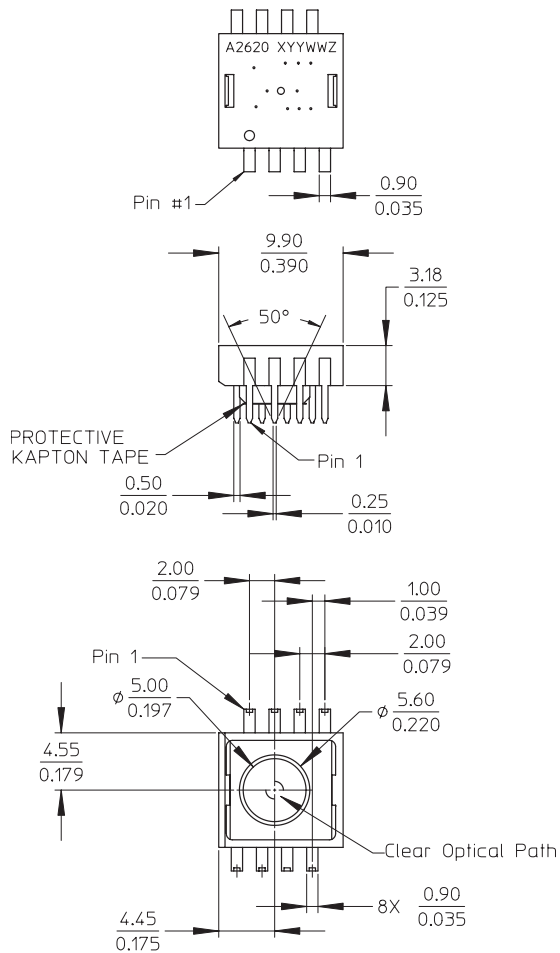
Figure 2. Package outline drawing.
