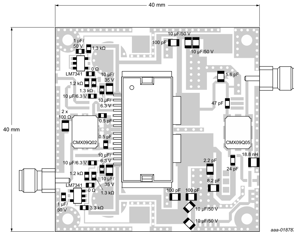
Fig 3. Component layout
