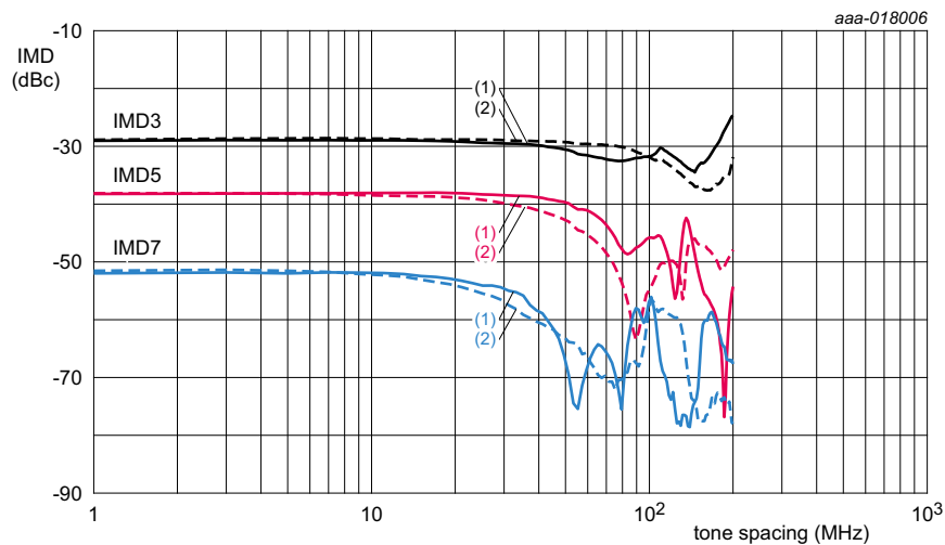
T_{\text{case}} = 25\text{ }^{\circ}\text{C} ; V_{\text{DS}} = 28\text{ V} ; I_{\text{DQ}} = 130\text{ mA} (carrier section); I_{\text{DQ}} = 4\text{ mA} (peaking section); f = 942.5\text{ MHz} . (1) IMD low (2) IMD high
