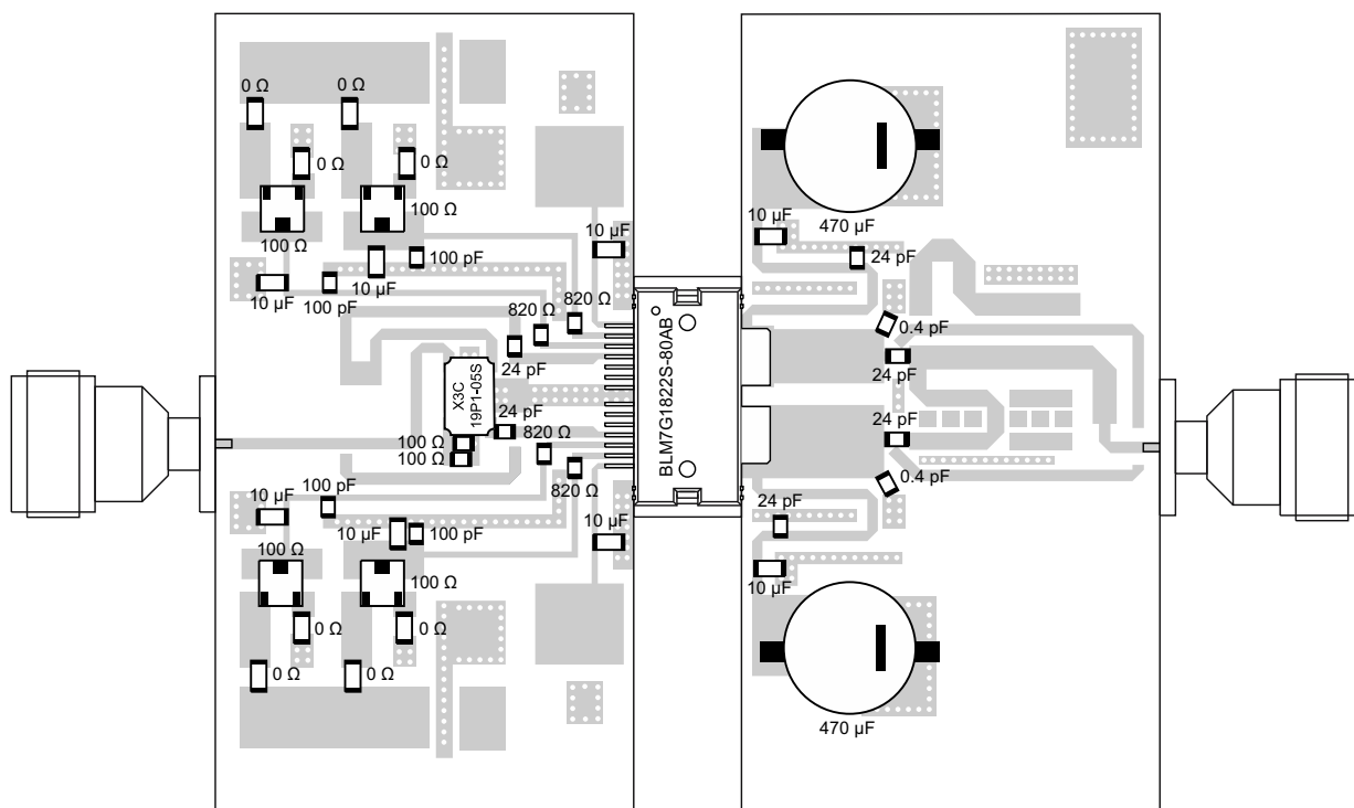
Fig 3. Component layout
